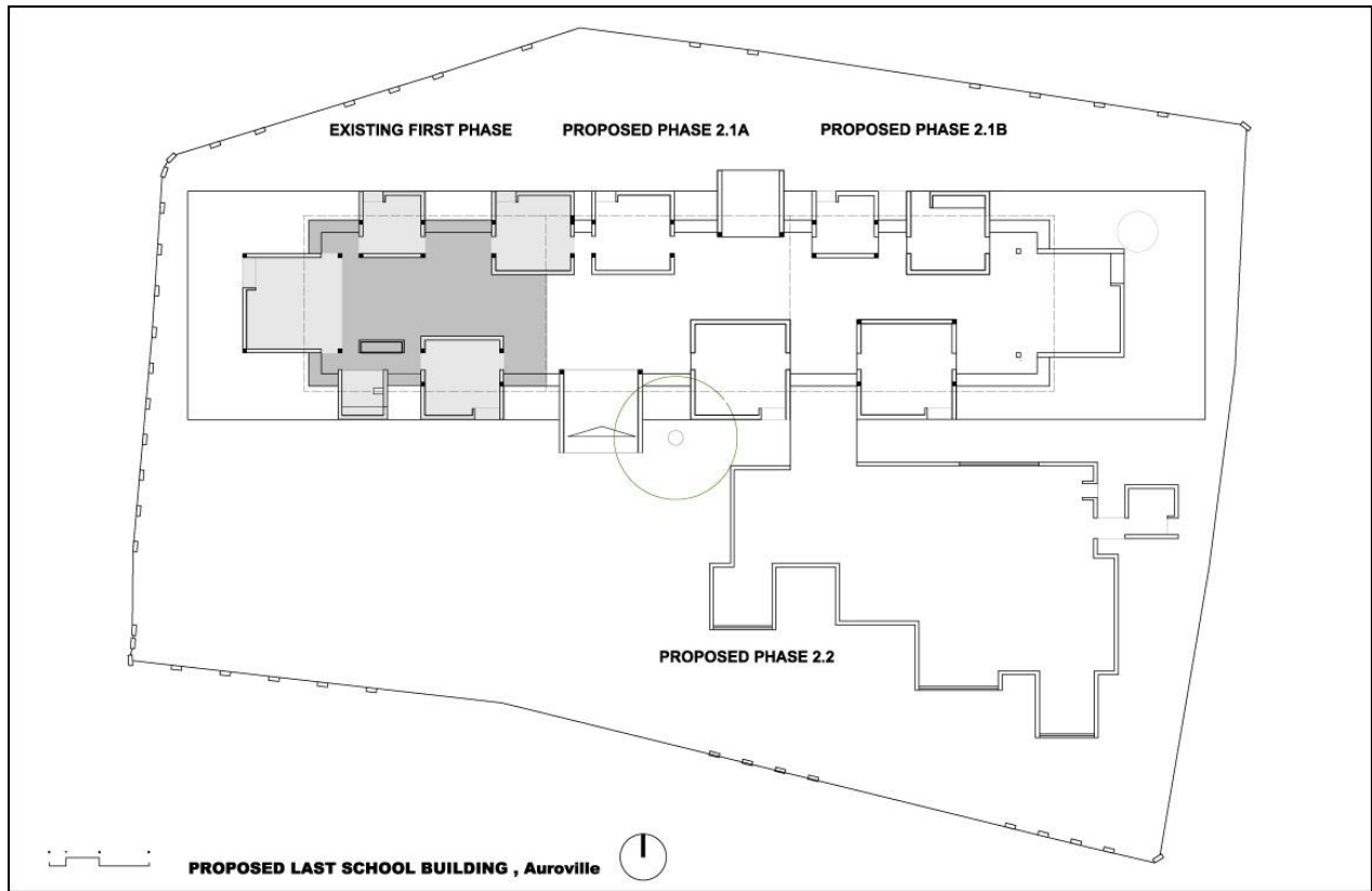
Groundfloor Plan
